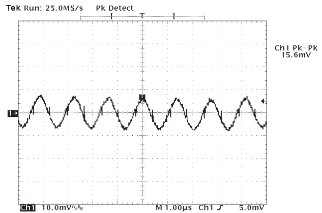
Figure 15: Typical Output Ripple
